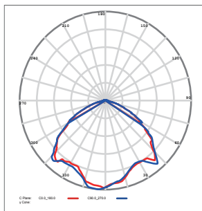
120 DEGREE (Tampere threaded glass)
